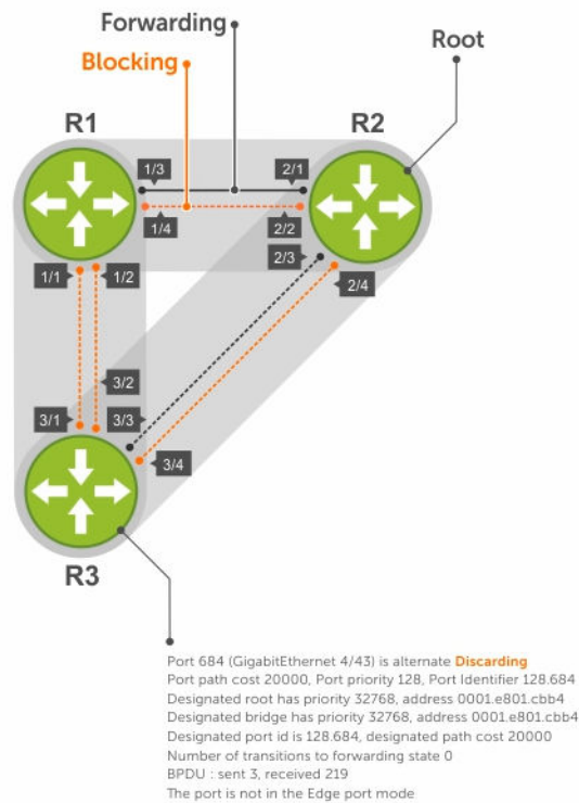
Figure 103. Rapid Spanning Tree Enabled Globally
